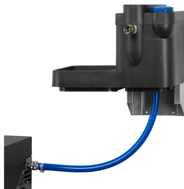
External Water Break Tank for up to 40 ltr/min.
